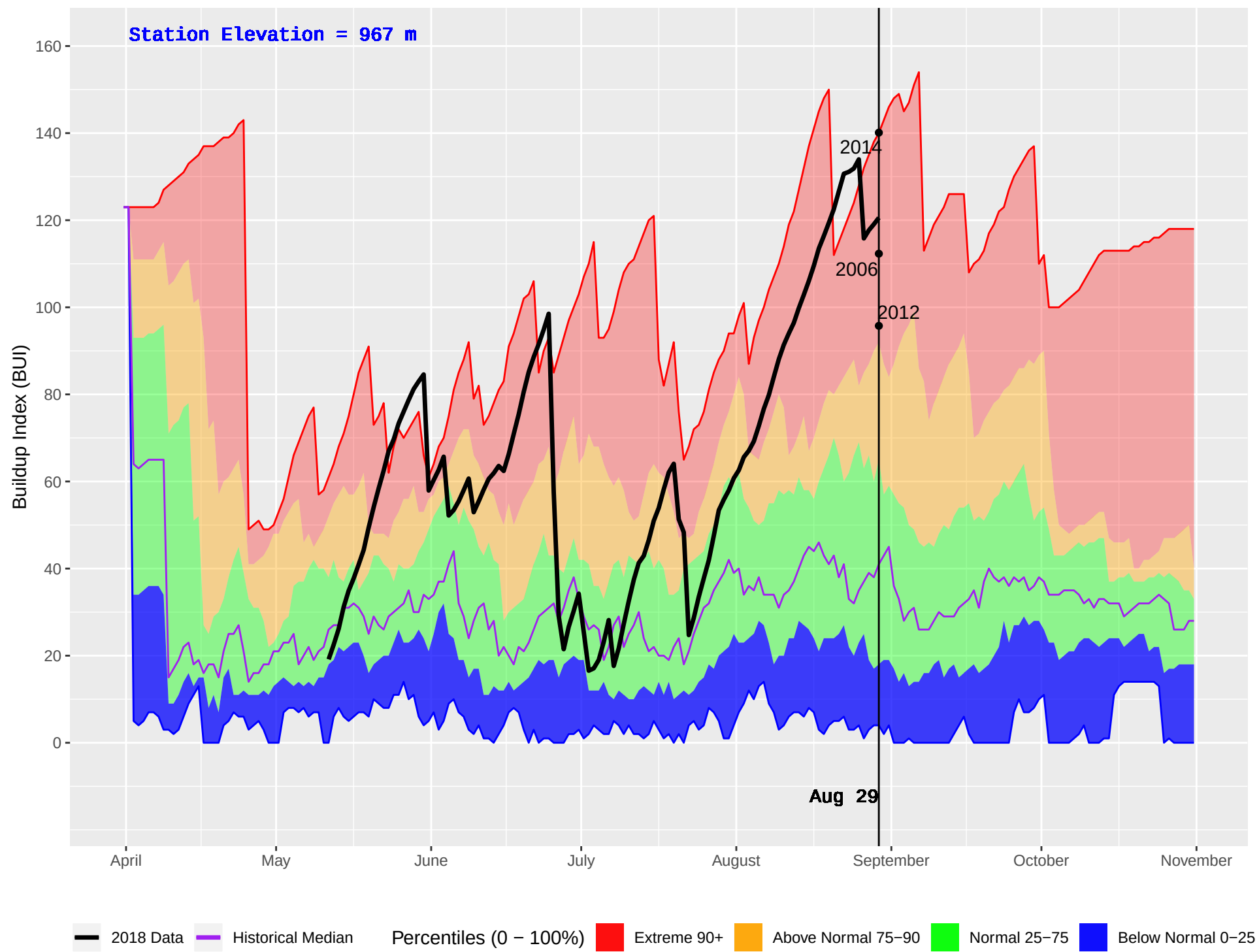
WONOWON (136) : Historical (1990–2016) and Current (2018) Daily Buildup Index (BUI)
