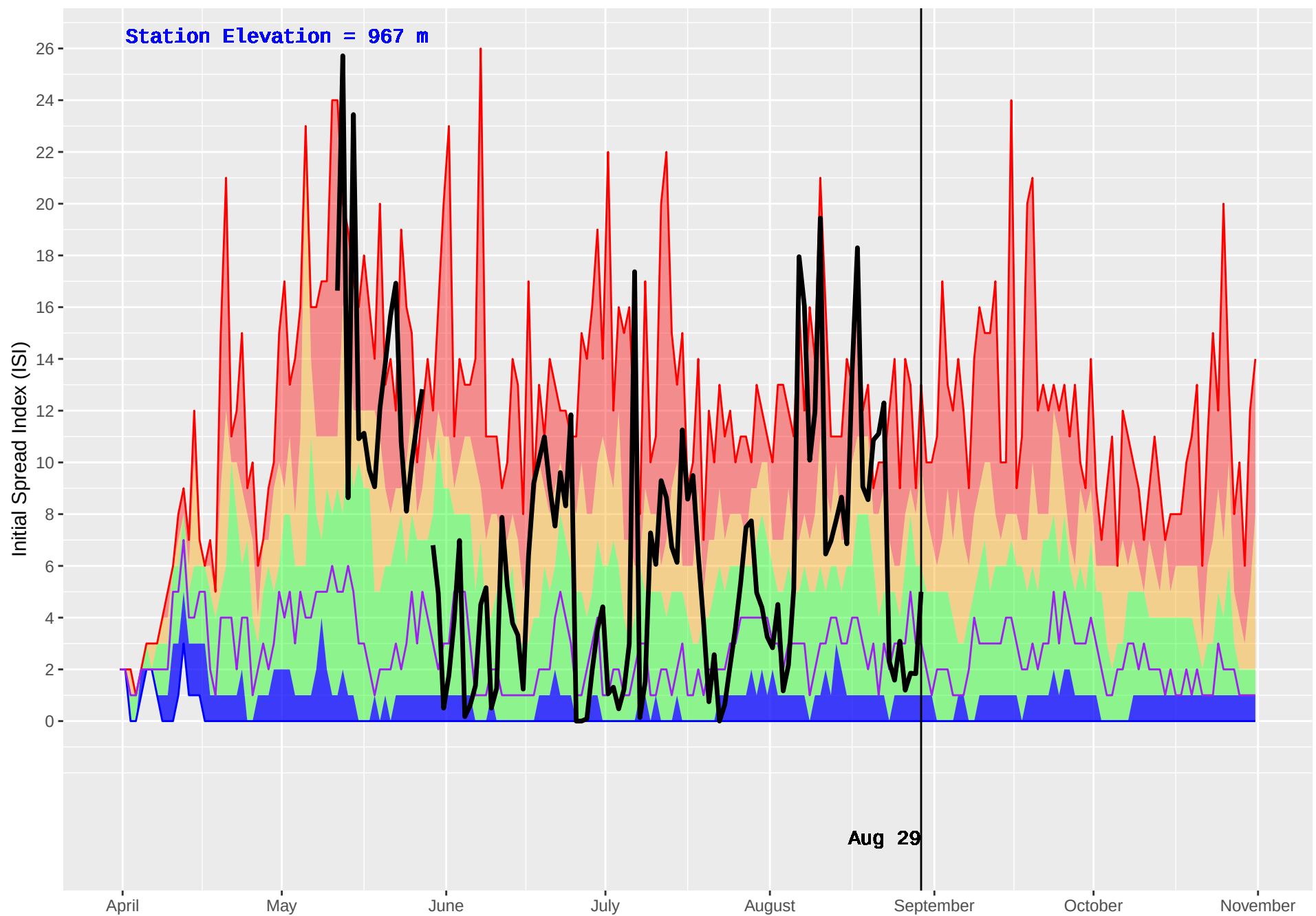
WONOWON (136) : Historical (1990–2016) and Current (2018) Daily Initial Spread Index (ISI)
