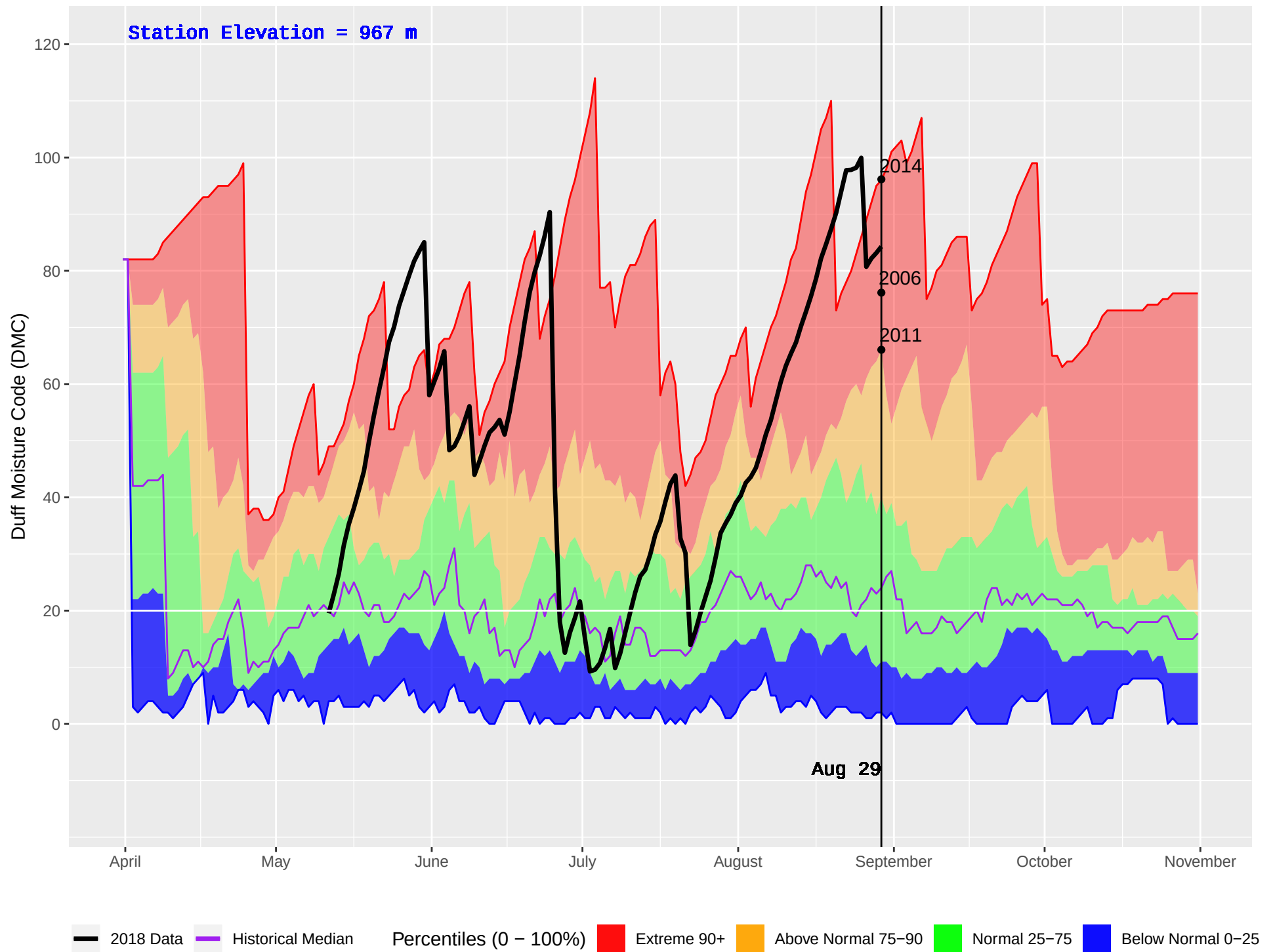
WONOWON (136) : Historical (1990–2016) and Current (2018) Daily Duff Moisture Code (DMC)
