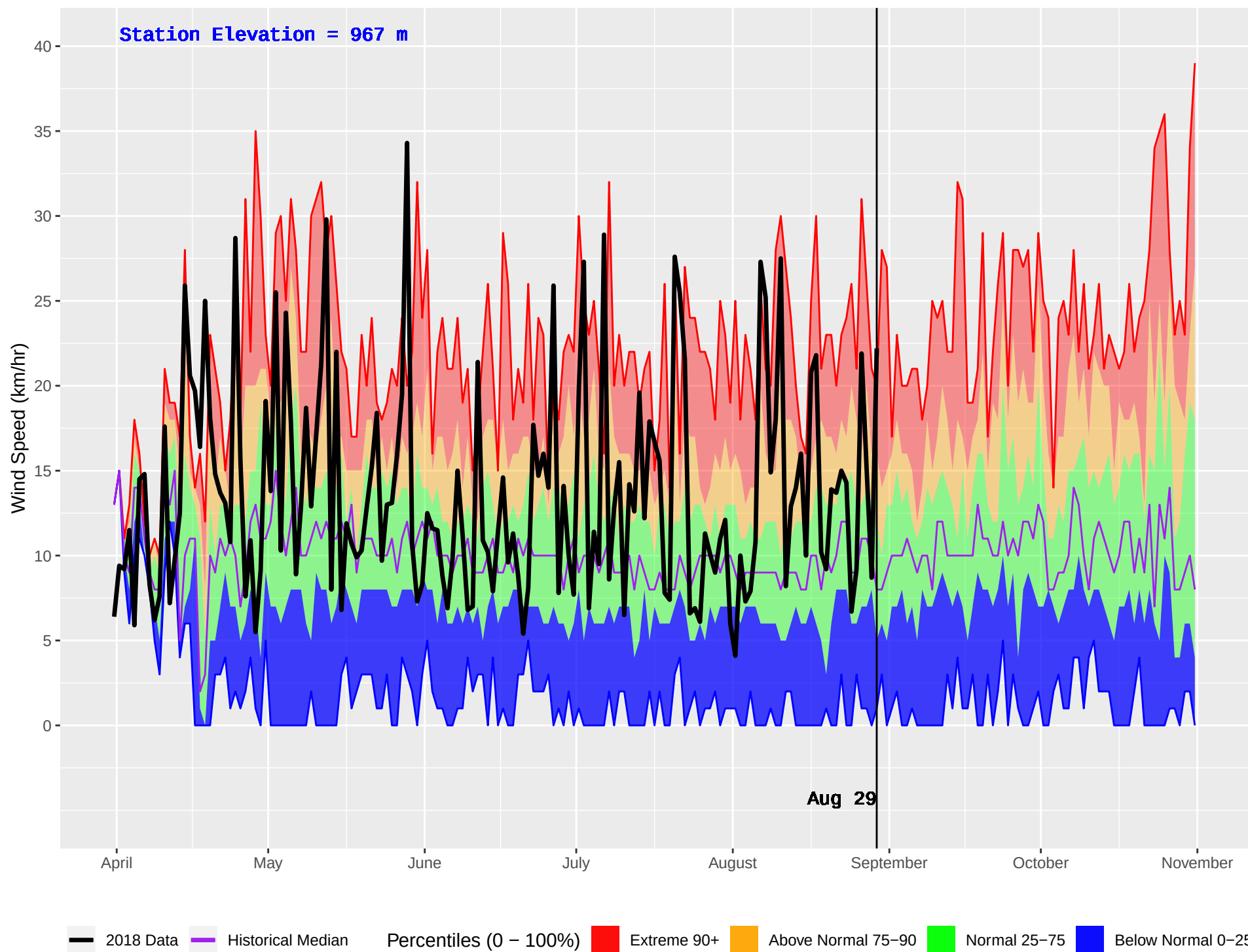
WONOWON (136) : Historical (1990–2016) and Current (2018) Daily Wind Speed
