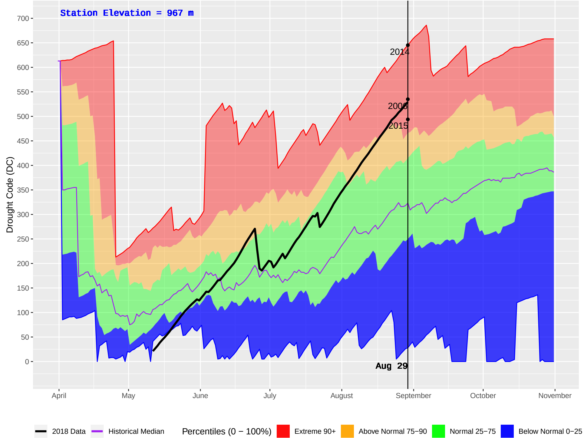
WONOWON (136) : Historical (1990–2016) and Current (2018) Daily Drought Code (DC)
