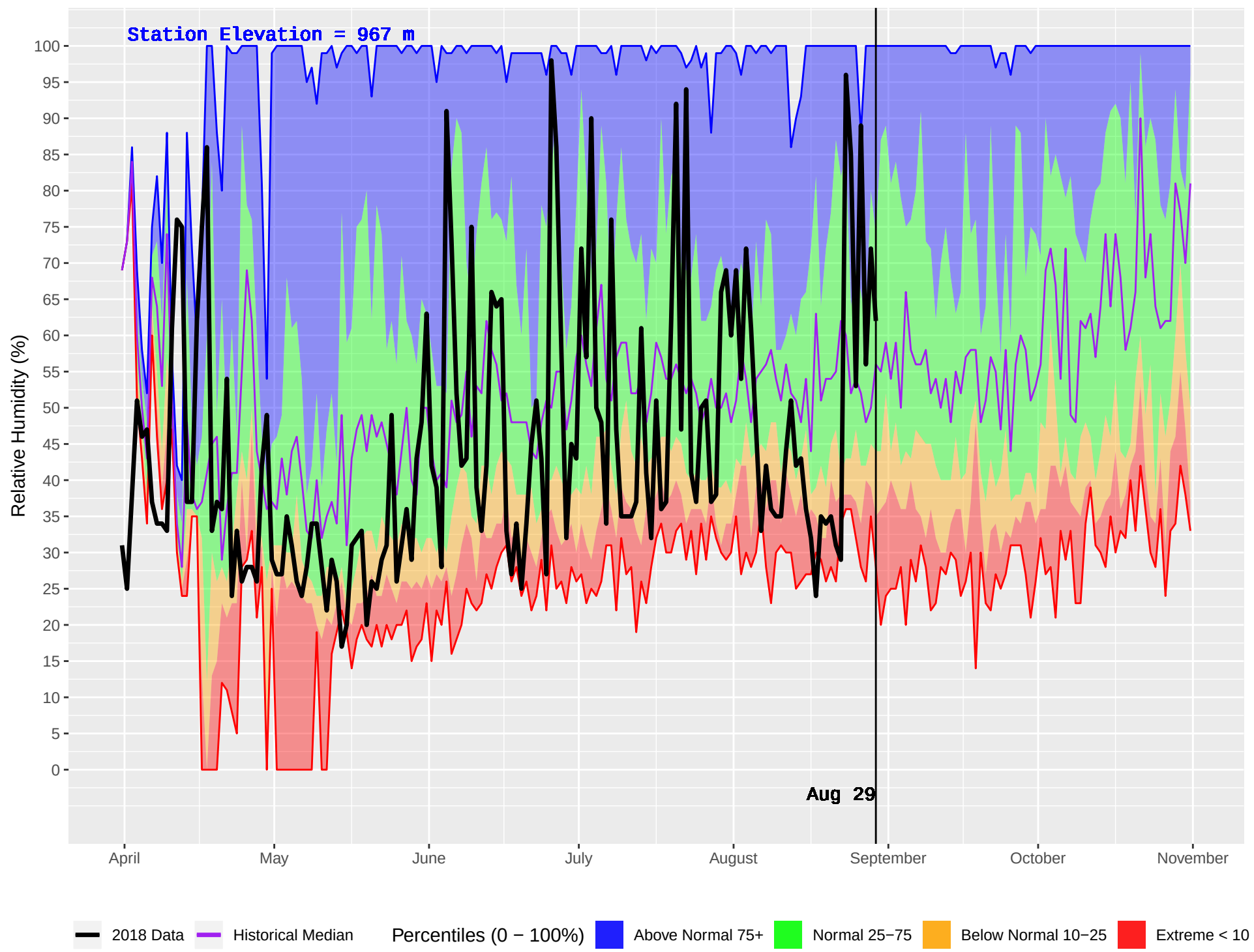
WONOWON (136) : Historical (1990–2016) and Current (2018) Daily Relative Humidity
