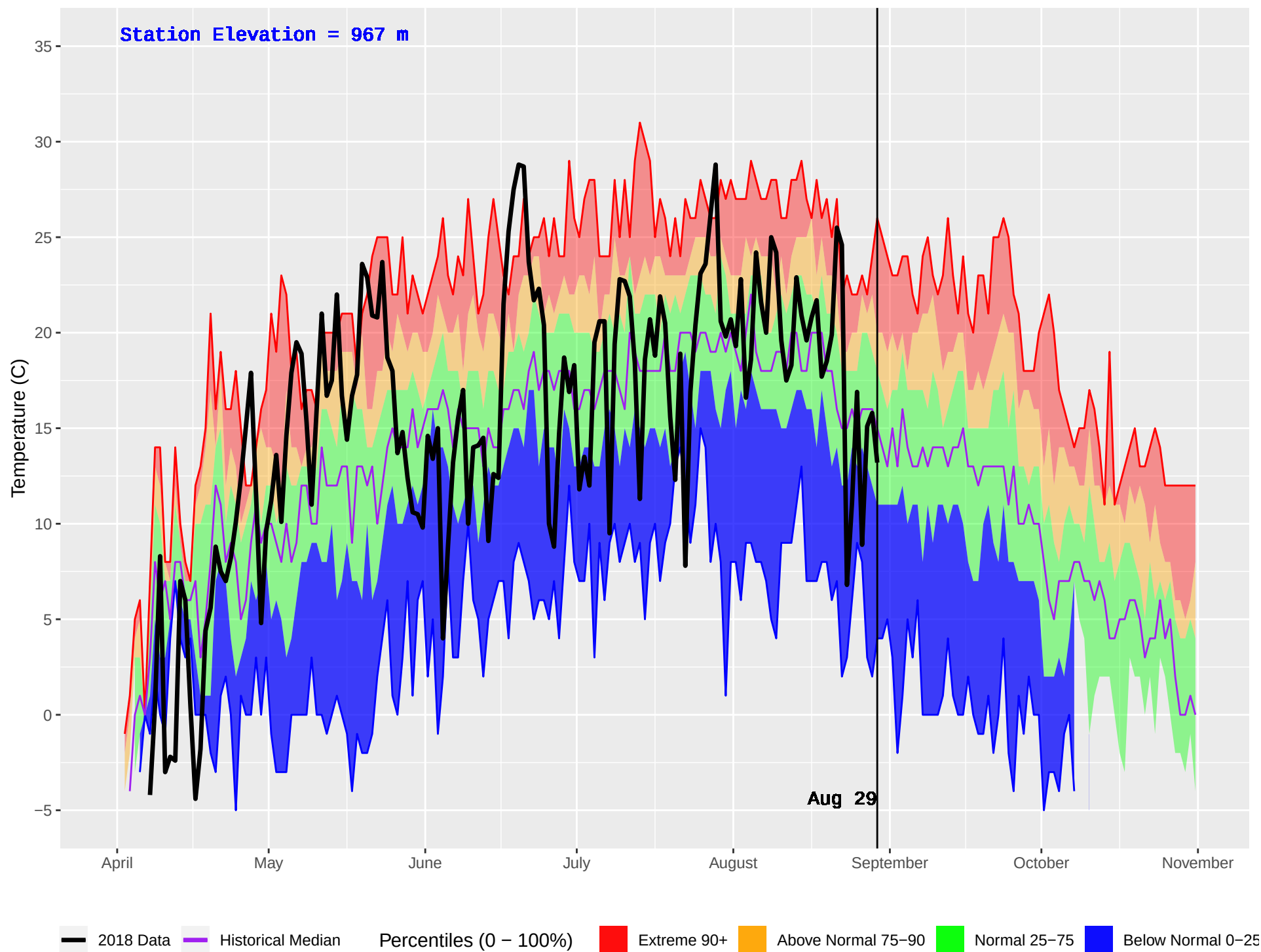
WONOWON (136) : Historical (1990–2016) and Current (2018) Daily Temperature
