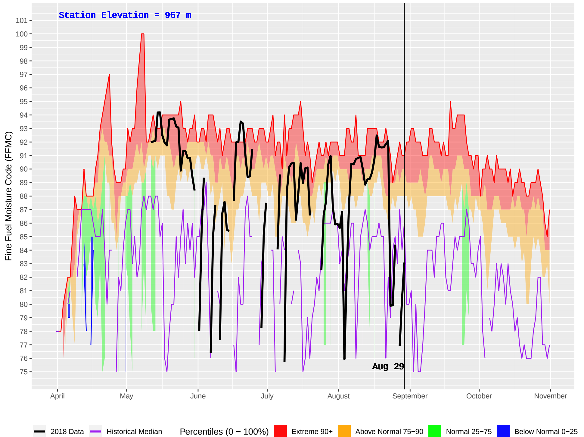
WONOWON (136) : Historical (1990–2016) and Current (2018) Daily Fine Fuel Moisture Code (FFMC)
