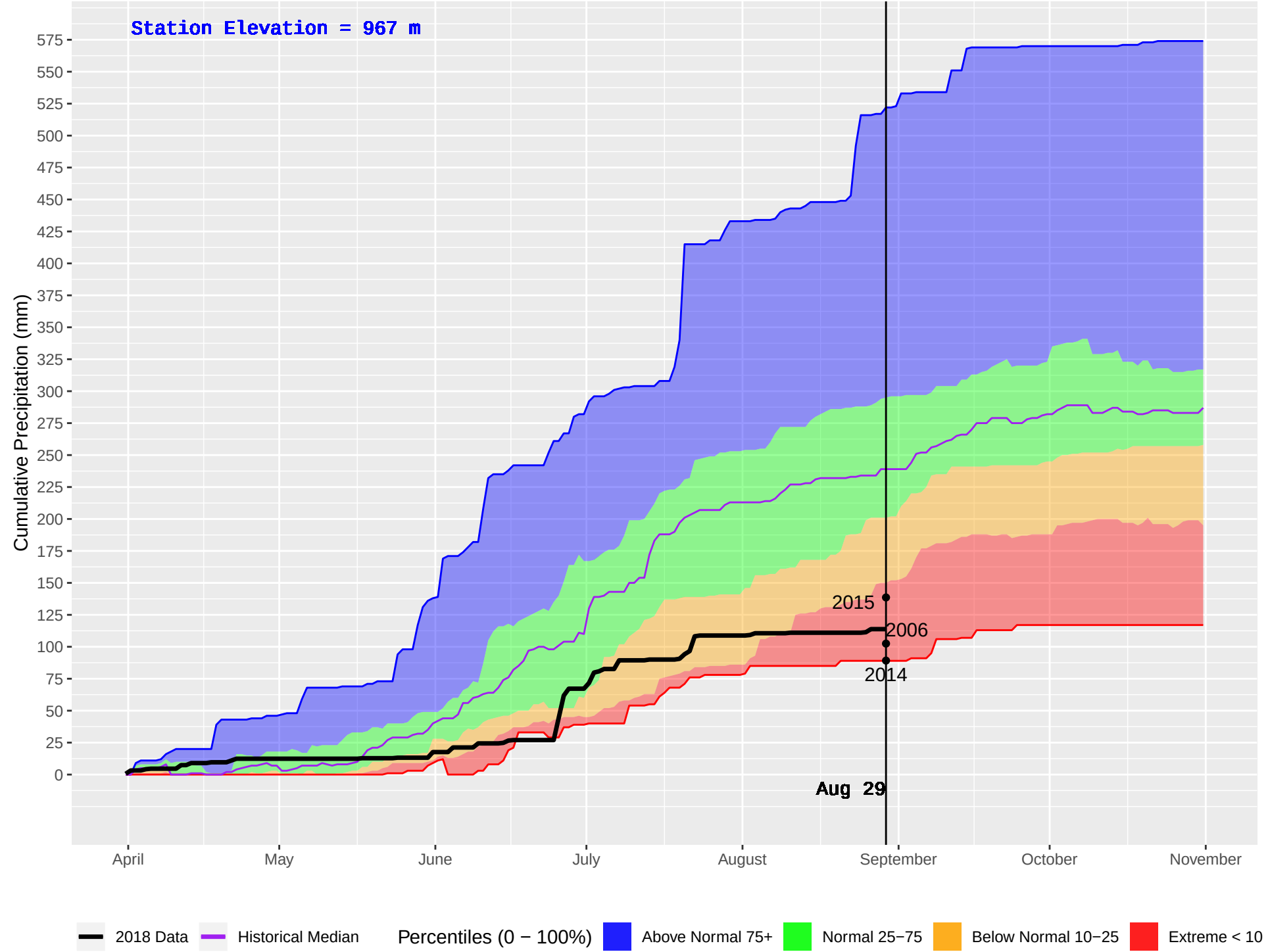
WONOWON (136) : Historical (1990–2016) and Current (2018) Daily Cumulative Precipitation
